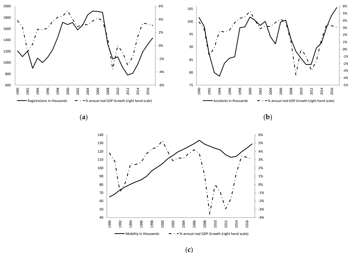
Figure 2. Spanish auto-market variables 1990–2017: (a) registrations M1+N1; (b) accidents; (c) mobility.
