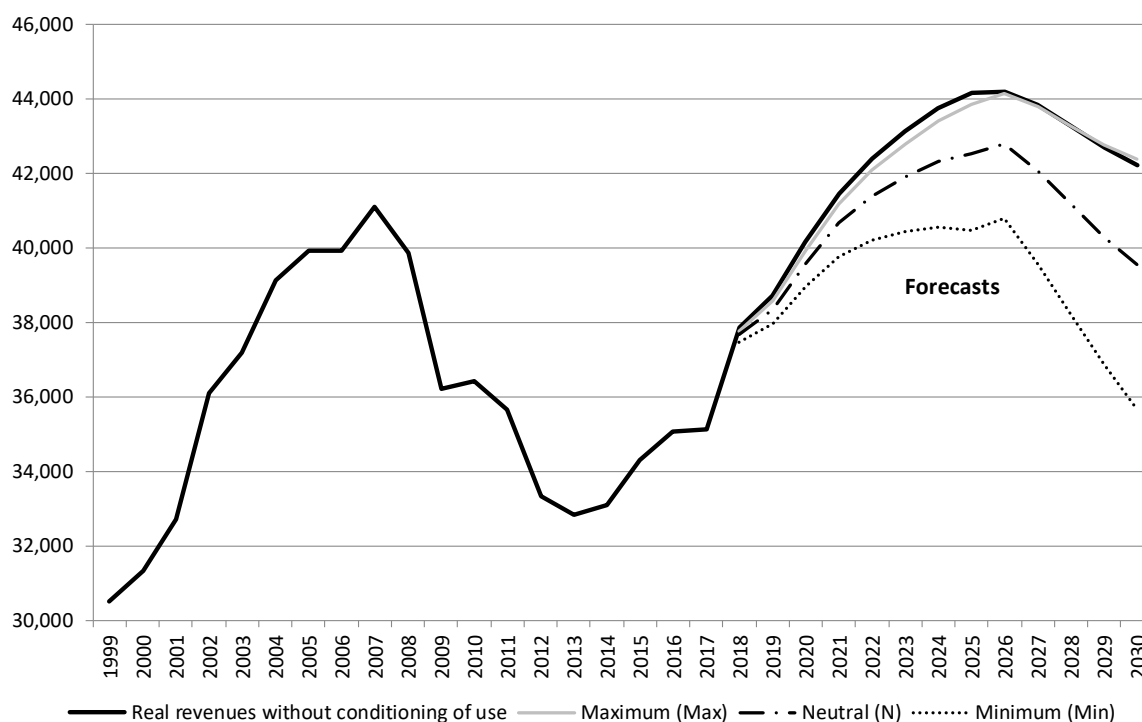
Figure 6. Forecasting automotive aftermarket's real revenues: 2018–2030.
