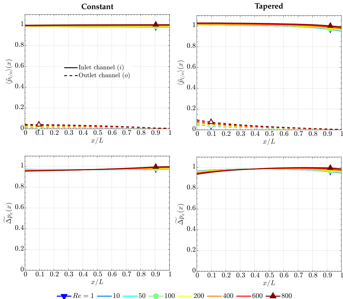
Figure 6. Variation of (top) the y -averaged pressure in the inlet and outlet channels, \langle \bar{p}_{i/o} \rangle(x) , and (down) the pressure drop across the electrode, \langle \Delta p_e \rangle(x) , as a function of the along-the-channel coordinate, x/L , for Re = 1 - 800 , corresponding to (left) the constant cross-section and (right) the tapered flow fields. Electrode permeability, K_e = 10^{-12} \text{ m}^2 ( \gamma \sim 10^{-2} ), and \Lambda = 26.67 .
