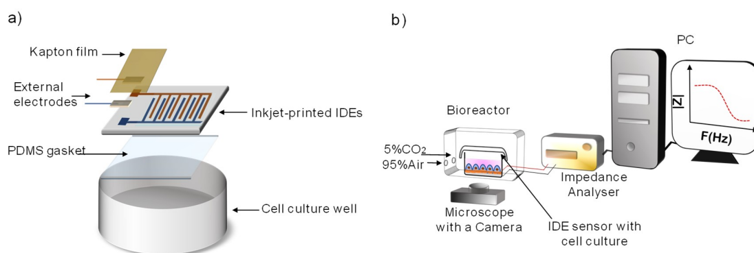
Figure 2. (a) Assembly and packaging of the IDE-based devices to perform impedance spectroscopy of cultured cells. (b) Schematic representation of the impedance-based biosensor system. The system consists of inkjet-printed IDE sensors, an IDEs-based chamber, an impedance analyzer, a microscope with an integrated bioreactor and a PC to control the images acquisition and the impedance recordings in real-time.
