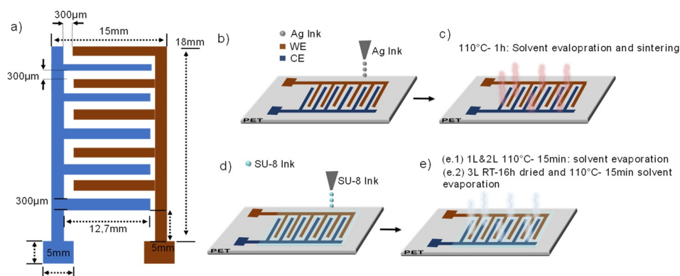
Figure 1. (a) Sketch and (b–e) manufacturing strategies for inkjet printing coplanar capacitors, showing the materials used and curing parameters for the development of the sensors.
