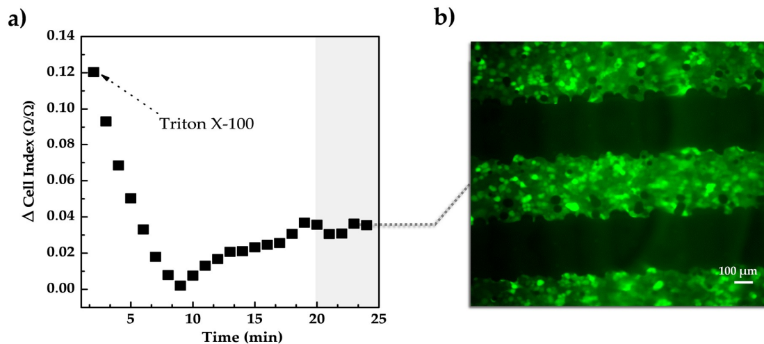
Figure 6. (a) Monitoring the addition of chemicals by impedance spectroscopy. Triton X-100 was added to the cell culture to destroy the bi-lipid membrane of the cells. The impedance drastically dropped in the first 10 min after the addition of the chemical. (b) Optically observation of the presence of cells under the sensors after 20 min of adding Triton X100.
