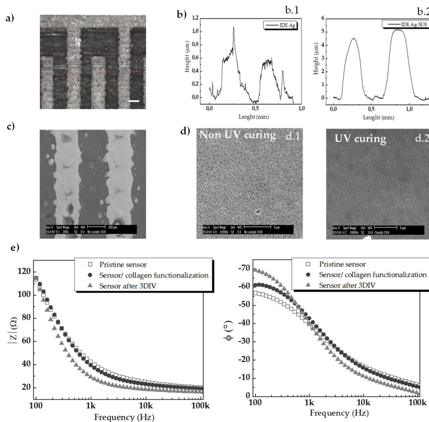
Figure 3. (a) Optical micrography of the inkjet-printed sensors (scale bar 100 \mu\text{m} ). (b) Surface profilometry of the two continuous inkjet-printed electrodes, revealing a thickness of a 0.6 \mu\text{m} for bare Ag electrodes (b.1) and 4 \mu\text{m} for passivated electrodes (b.2). (c) SEM micrography of the inkjet-printed sensor surface in a top view (scale bar 200 \mu\text{m} ). (d) The effect of UV curing on the SU-8 passivation layers showed an increase in the smoothness of the outmost layer. UV treated samples showed a smoother surface (d.2) compared with non-treated samples (d.1). (e) Electrical performance of pristine inkjet-printed sensors, sensors with collagen functionalization, and sensors after three days in vitro with HaCaT cell cultures. Magnitude of the impedance (left) and phase (right).
