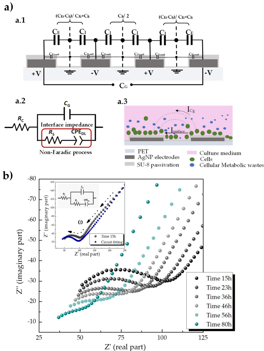
Figure 7. (a) Equivalent circuit model to fit the impedance measured in a non-faradic analysis. (a.1) Example of the electrical equivalent applying partial capacitance techniques of a sensor with four electrodes and considering the effect of finite multilayer passivation on top of the electrodes on the static capacitance. (a.2) Electric circuit model of the IDEs with cells in a culture medium modeling the resistivity of the culture medium, R_c , the capacitance of the IDEs, C_g , and the impedance of the surface interface. The presence of cells is modeled by a constant phase element, CPE_{DL} , and a resistance R_s . (a.3) Schematic representation of the biophysical interpretation of such an equivalent circuit model showed in a.1. The total current can pass through the interface as a sum of the contributions from the geometrical capacitance of the IDEs (curved arrow I_{Cg} ) and the non-faradic process that takes place in the interface of the electrodes due to the presence of cells (straight arrow I_{surface} ). The dashed lines in the schematic represent the electric field generated due to the nature of the interdigitated electrodes. Green circles represent the HaCaT-GFP cells seeded on the sensors while the blue dots represent the cellular wastes as a result of their growth medium's consumption. (b) Nyquist plot of experimental impedance spectra for monitoring cell detachment and death during 80h period. The inset plot shows the measured impedance and the corresponding fitting with the circuit model at time 15 h. Each point in the Nyquist plot represents the impedance at one frequency, in which higher frequencies appear closer to the origin (i.e., lower values of the real part in the magnitude of the impedance).
