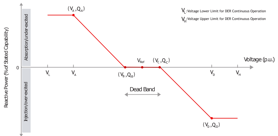
Figure 1. Voltage—Reactive Power response example [18].
