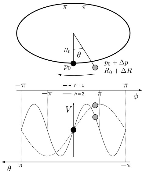
Figure 2.1: Illustration of the azimuthal angle \theta , radius R , momentum p and phase \phi variables. The phase is to be interpreted with respect to the RF voltage for two harmonics: h = 1 and h = 2 in this example. Note that the phase and azimuth angles are the opposite sign following the usual convention E.g. [123, 124].
