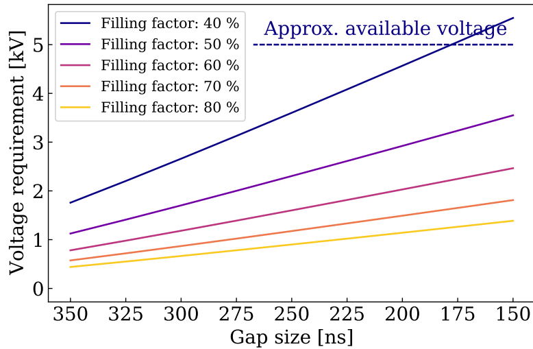
Figure 3.1: Peak voltage requirement for the ideal case of emittance preservation during re-bucketing.
