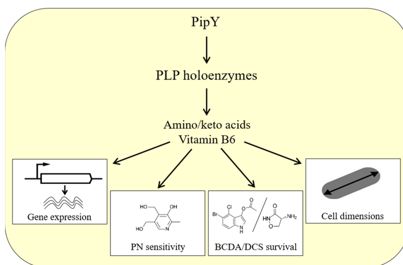
Figure 3. Roles of PipY and affected processes in cyanobacteria. PipY would function as a PLP storage and delivery module, and influence the activity of PLP-holoenzymes, which in turn affect the amino/keto acid pool and the processes responsive to (some of) these metabolites. Phenotypes dependent on PipY include the control of gene expression, PN sensitivity, survival in the presence of antibiotics targeting PLP-holoenzymes, and altered cell dimensions. Abbreviations: PN, pyridoxine; DCS, D-cycloserine.
