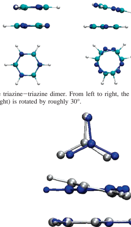
Figure 5. Triazine–triazine–NO 3 − complex with relative orientation of the rings of 60° optimized within DFT/BLYP-DCACP (gray). In blue, we show the starting symmetrical geometry.
