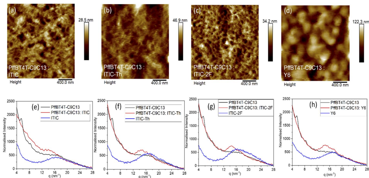
Fig. 3 AFM images of topography for (a)PffBT4T-C9C13:ITIC, (b)PffBT4T-C9C13:ITIC-Th, (c) PffBT4T-C9C13:ITIC-2F, and (d)PffBT4T-C:Y6. Scale bars are 400 nm. GIXRD (normalised per absorption) for pristine PffBT4T-C9C13 film and (e) ITIC and PffBT4T-C9C13: ITIC (1 : 1.2) film (f) ITIC-Th and PffBT4T-C9C13: ITIC-Th (1 : 1.2) film (g) ITIC-2F and PffBT4T-C9C13: ITIC-2F (1 : 1.2) film (h) Y6 and PffBT4T-C9C13: Y6 (1 : 1.2) film.
