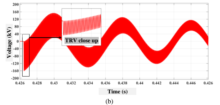
Fig. 2. a) TRV of FCB without using SSSR, b) TRV close-up view
