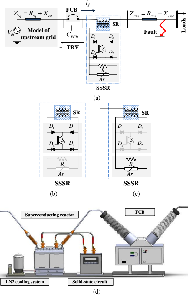
Fig.4. SSSR structure and operation, a) SSSR Configuration, b) SSSR model in normal condition, c) SSSR model in fault condition. d) 3D scheme of SSSR configuration
