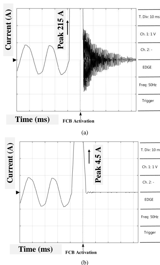
Fig. 14. Measured signal of fault current (probe X25), a) without SSSR installation b) with SSSR operation
