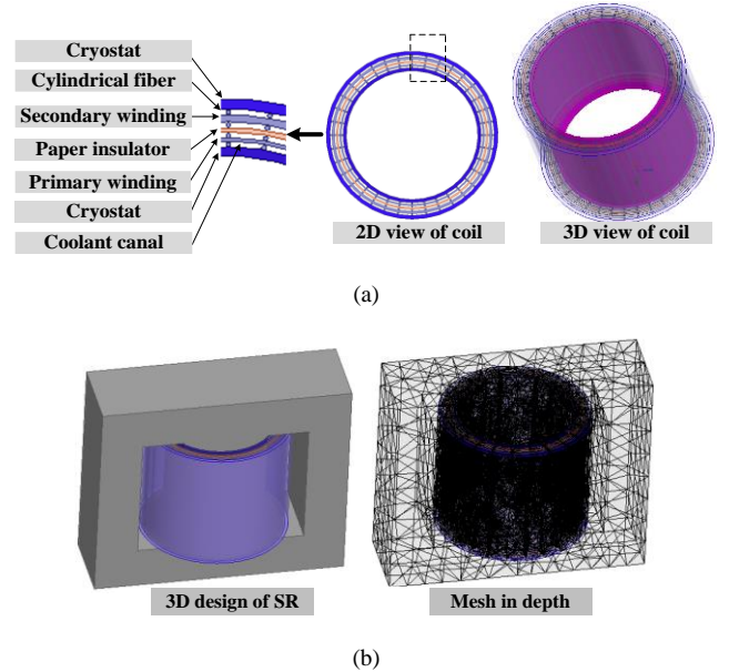
Fig. 10. a) Geometric view of SR coil, b) 3D design of SR and mesh sections
