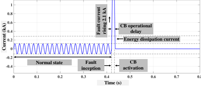
Fig. 8. a) line fault current considering SSSR effect
