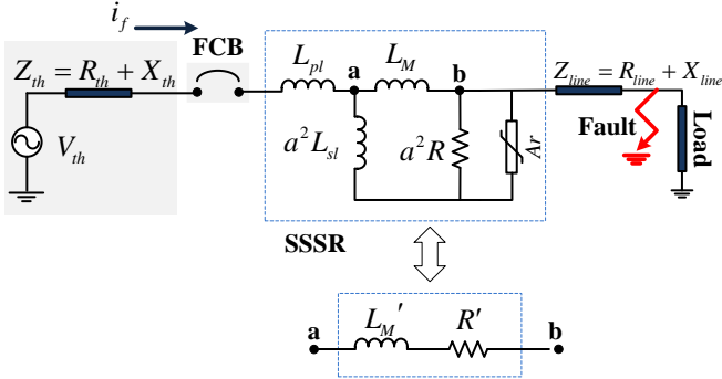
Fig. 6. The SSSR model under fault condition
