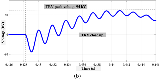
Fig. 7. a) TRV of FCB considering SSSR effect, b) close-up view of TRV
