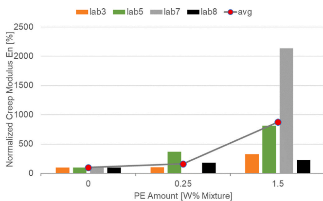
Fig. 14. Normalized Creep Modulus as a function of amount of PE normalized with respect to reference.
