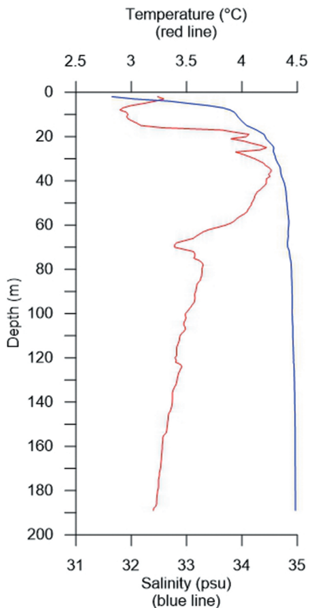
Figure 3. Temperature (red line) and salinity profile (blue line) from CTD (conductivity, temperature and density) cast carried out prior to coring, 2 August 2016 (Husum and Wold 2016).
