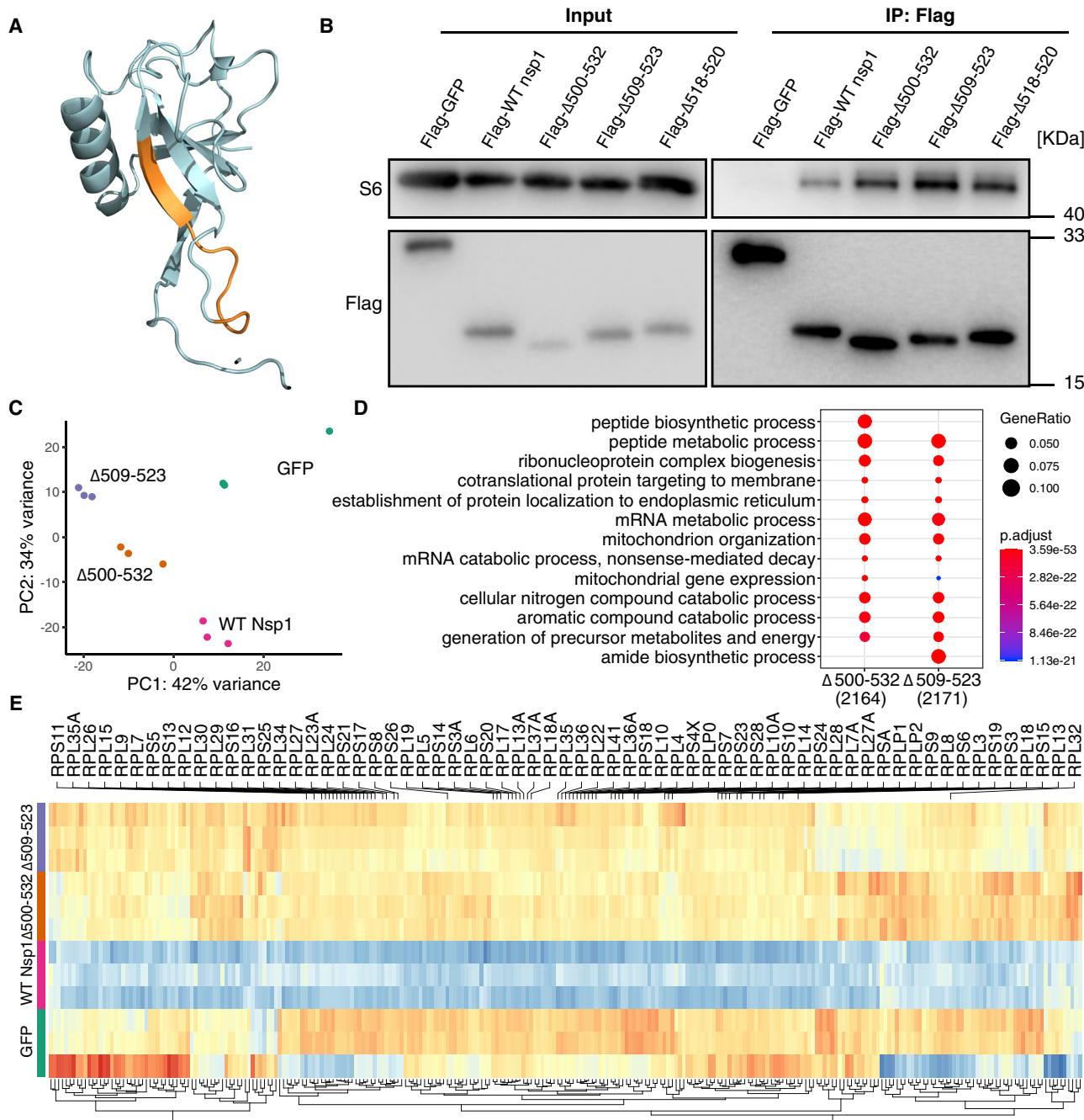
Figure 5. Nsp1 mutants retained ribosomal binding ability while affecting mRNA metabolic process
