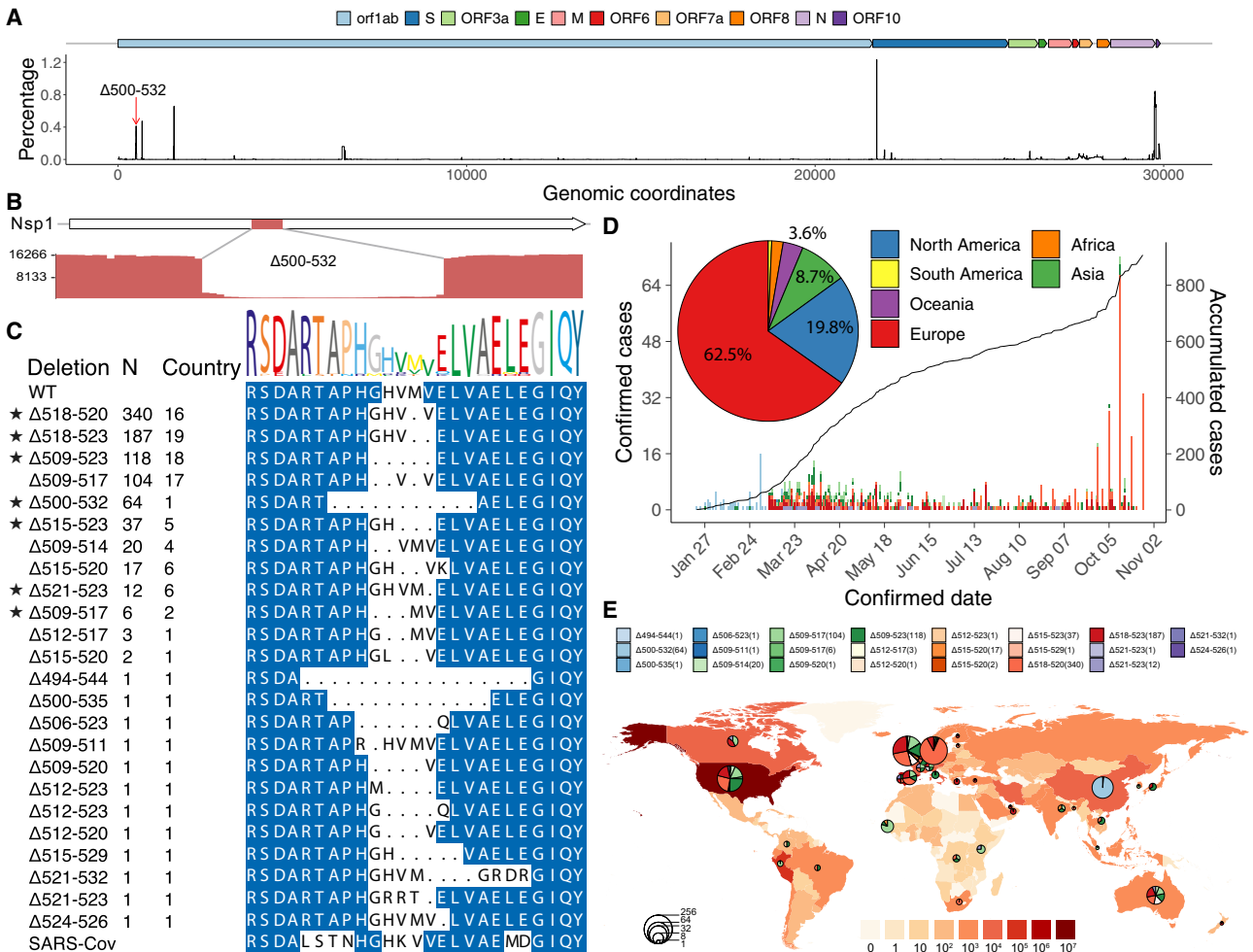
Figure 4. Prevalence of deletion variants in the 500-532 locus in SARS-CoV-2 genome
