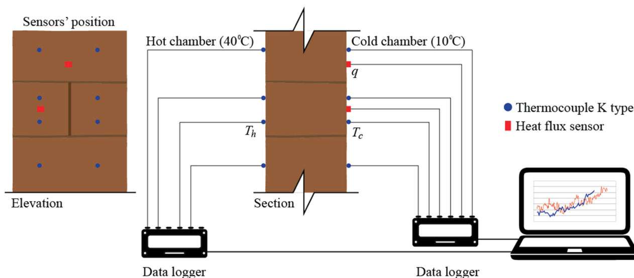
Figure 7. Configuration of the sample wall and position of the sensors.
