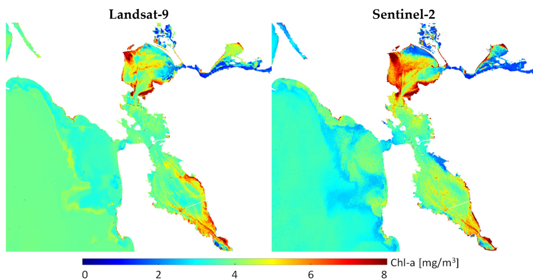
Figure 14. Chl-a maps derived from Landsat-9 and Sentinel-2 imagery in San Francisco Bay based on NN regression model.
