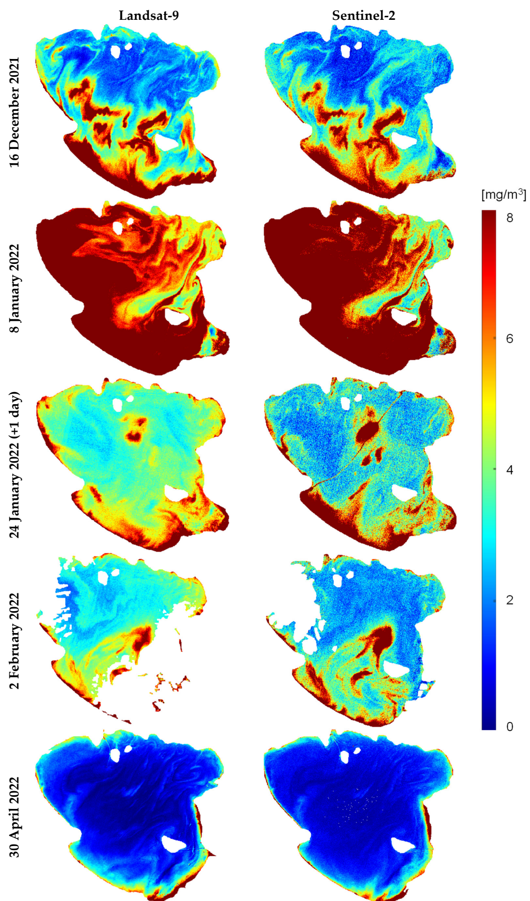
Figure 9. Chl-a maps derived from Landsat-9 and Sentinel-2 imagery in Lake Trasimeno using BOMBER.
