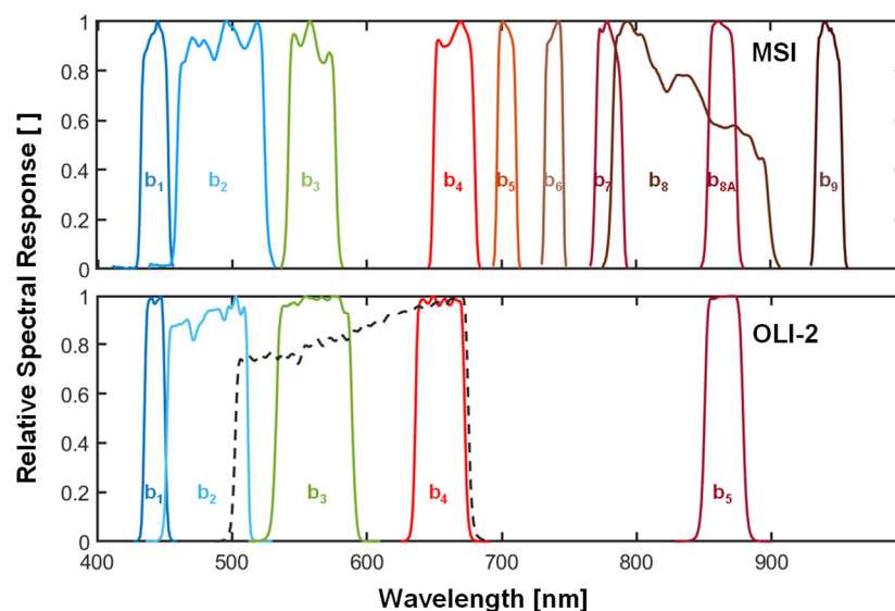
Figure 4. Relative spectral response of OLI-2 and MSI onboard Landsat-9 and Sentinel-2, respectively. The band numbers are provided for each sensor, and the gray dashed line shows Landsat-9 panchromatic band.
