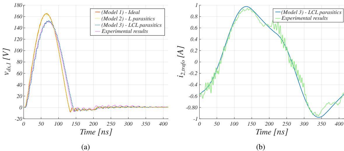
Fig. 7: Experimental and simulated waveforms with an input voltage of 30 V and a switching frequency of 2.415 MHz. (a) shows the drain-source voltage and (b) shows the secondary side transformer current.
