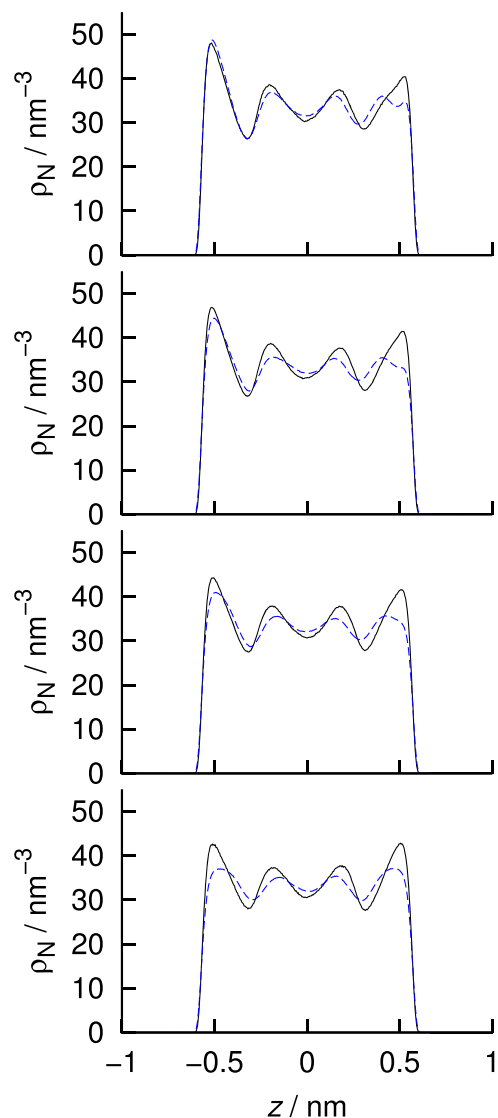
FIG. 3. Density distributions of BK3 (black solid curves) or SPC/E (blue dashed curves) molecules across the nanopore between a pair of smooth walls at separation 1.64 nm in equilibrium with the bulk phase at ambient conditions in the absence (bottom) or presence of perpendicular fields (directed from the left to the right wall) of strengths (from bottom to top) D_z = 0.0, 0.00885, 0.0177, and 0.0266 \text{ C m}^{-2} . Statistical uncertainties are of the order of \pm 1\% .
