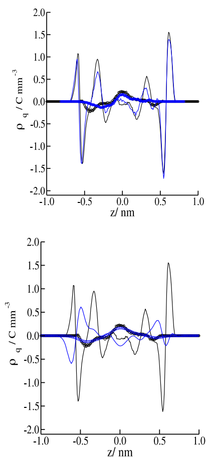
FIG. 12. Top: The average charge density profiles due to BK3 (black lines) or SPC/E (blue lines) water molecules and polarizable NaCl ions in BK3 water (black circles) or JC ions in SPC/E (blue circles) solvent nanopore with smooth walls under electric displacement field D_z = 0.0177 \text{ C m}^{-2} , corresponding to a field-free reservoir with a NaCl concentration of \sim 2 \text{ mol kg}^{-1} . Bottom: Comparison between the profiles for BK3-AH solutions from the top graph (black lines and symbols) and the results obtained in the BK3-AH system (blue lines and symbols) when explicitly accounting for the Gaussian charge distributions of mobile charges (blue lines and symbols).
