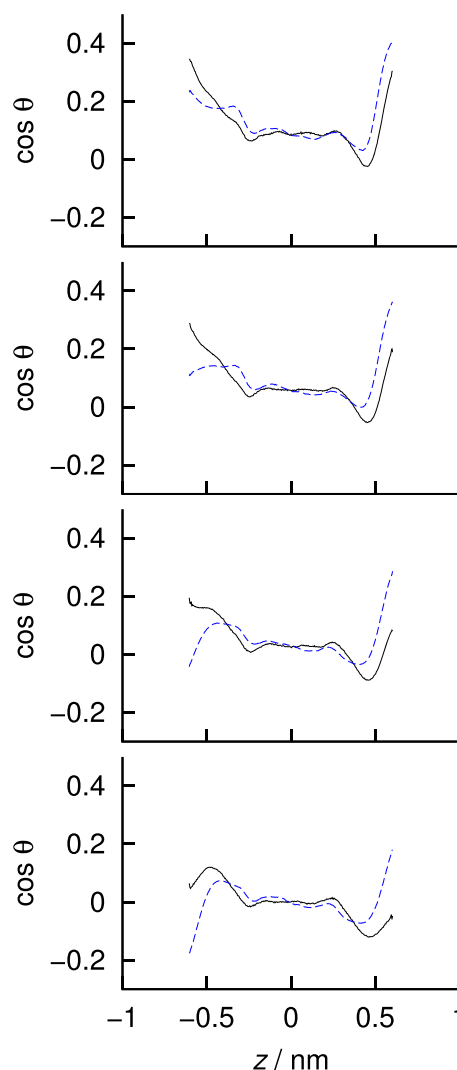
FIG. 5. The average orientation of molecular dipoles of BK3 (black solid curves) or SPC/E molecules (blue dashed curves) measured in terms of the angle \theta between the dipole and the direction of the field (normal to the walls) as functions of the position inside the pore at electric displacement fields D_z = 0.0, 0.00885, 0.0177, and 0.0266 \text{ C m}^{-2} (from bottom to top) between smooth walls in GCMC simulations maintaining equilibrium between the pore and a bulk reservoir of water at ambient conditions.
