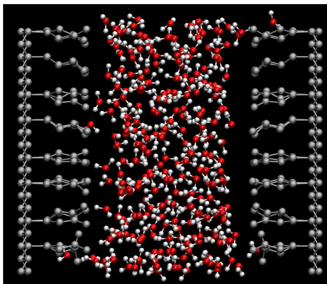
FIG. 1. Snapshot of confined BK3 water film between alkyl-coated graphene plates subject to perpendicular electric field. Field E_z spanning the aqueous film (average strength \sim 0.08 \text{ V nm}^{-1} ) supports occasional penetrations of water molecules into the alkyl brush.
