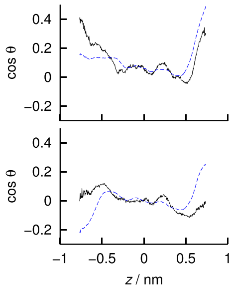
FIG. 8. The average orientation of molecular dipoles of BK3 (black solid curves) or SPC/E molecules (blue dashed curves) measured in terms of the angle \theta between the dipole and the direction of the field (normal to the walls) as functions of the position inside the pore at fields D_z = 0.0 \text{ C m}^{-2} (bottom) and D_z = 0.0266 \text{ C m}^{-2} (top) between butyl-coated walls in GCMC simulations maintaining equilibrium between the pore and a bulk reservoir of water at ambient conditions.
