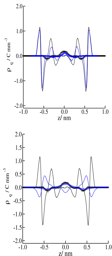
FIG. 11. Top: The average charge density profiles due to BK3 (black lines) or SPC/E (blue lines) water molecules and polarizable NaCl ions in BK3 water (black circles) or JC ions in SPC/E (blue circles) solvent in a field-free nanopore with smooth walls and an equilibrium reservoir concentration of \sim 2 mol \text{kg}^{-1} . Bottom: Comparison between the profiles for BK3-AH solutions from the top graph (black lines and symbols) and the results obtained in the same system when explicitly accounting for the Gaussian charge distributions of the BK3-AH system. Overlapping Gaussian distributions reduce the density amplitudes of water and visibly shift the extrema of water contribution. A slight smoothing of the salt charge distribution is present.
