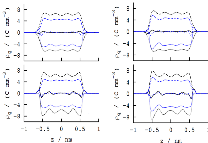
FIG. 10. The H (long-dashed curves) and O (dotted curves) contributions to local charge density \rho_q(z) for BK3 (black curves) and SPC/E (blue curves) water models and total charge-density profiles of BK3 (solid black curves) or SPC/E molecules (short-dashed blue curves) as functions of the position inside the pore between smooth walls in GCMC simulations maintaining equilibrium between the pore and a bulk reservoir of water at ambient conditions. The left graphs are obtained in the absence and the right ones in the presence of electric field of strength D_z = 0.0266 \text{ C m}^{-2} . Individual contributions from oxygen and hydrogen atoms greatly exceed the total densities. Charge densities are calculated by placing entire charges at charge site positions (bottom) or by explicitly accounting for the correct Gaussian charge distributions in the BK3 model (top). The former method shows small differences between the two models, whereas the actual densities due to the Gaussian charges in the BK3 model feature smoother profiles with reduced amplitudes and a considerable shift of the extrema relative to the distributions of point-charges.
