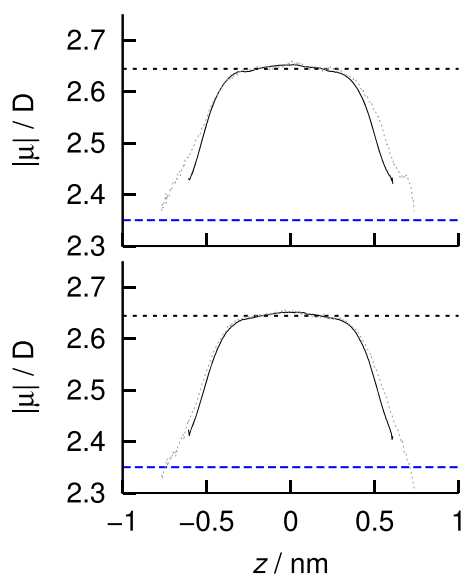
FIG. 4. The average magnitude of the molecular dipoles of BK3 (solid curves) molecules as functions of the position inside the pore in the absence (black solid curves) or presence of electric displacement field of strength 0.0266 \text{ C m}^{-2} (gray dotted curves) between smooth (bottom) or molecular (butyl-coated) walls (top) in GCMC simulations maintaining equilibrium between the pore and a bulk reservoir of water at ambient conditions. Horizontal lines correspond to bulk values of the dipoles of BK3 (black dashed lines) and SPC/E (blue dashed lines) molecules.
