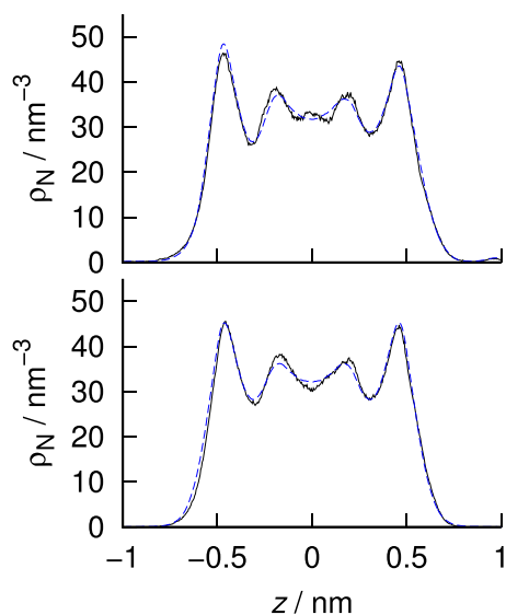
FIG. 7. Density distributions of BK3 (black solid curves) or SPC/E (blue dashed curves) molecules across the nanopore between a pair of butyl-coated graphene walls at separation 2.81 nm in equilibrium with the bulk phase at ambient conditions in the absence (bottom) or presence of perpendicular field (directed from the left to the right wall) of strength D_z = 0 (bottom) or 0.0266 \text{ C m}^{-2} (top). Statistical uncertainties are of the order of \pm 1\% .
