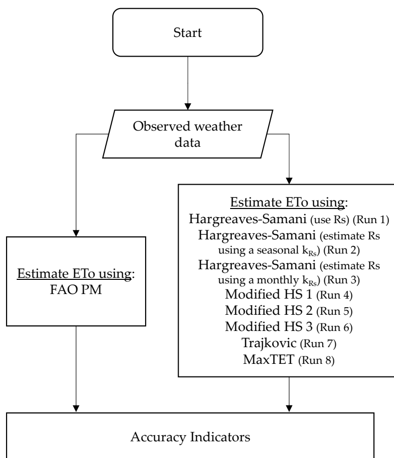
Figure 5. Flow chart presenting the example application runs performed with ETo Tool.
