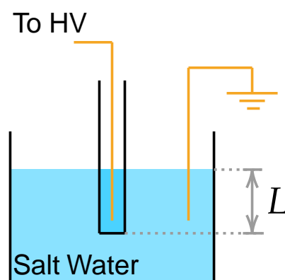
Figure 4.6: Setup of resistivity measurement. The glass tube is filled with and immersed in the solution to depth L . A voltage is applied across the glass allowing measurement of the current through its volume.
