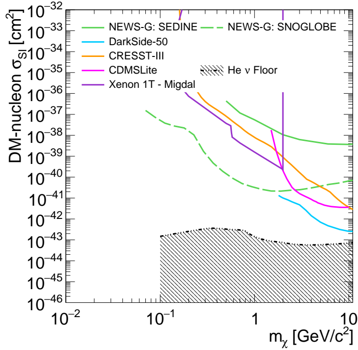
Figure 3.21: Projected 90% CL upper limit on the spin-independent DM-nucleon interaction cross section as a function of DM mass projected for SNOGLOBE. The neutrino floor is shown for helium [74]. Experimental exclusion limit measurements for SEDINE [144], and other direct DM experiments, DarkSide-50 [148], CRESST-III [149], CDMSlite [93] and Xenon-1T [104], are given for comparison.
