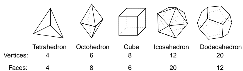
Figure 4.14: The five platonic solids.
