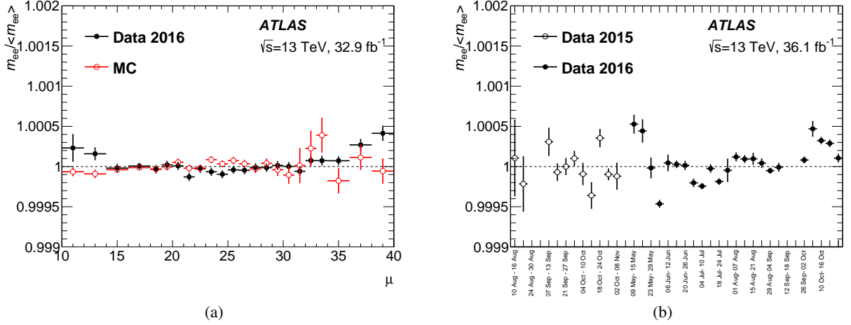
Figure 10: Relative variation of the peak position of the reconstructed dielectron mass distribution in Z \rightarrow ee events (a) as a function of the average number of interactions per bunch crossing for the 2016 data and (b) as a function of time over the full 2015 and 2016 data-taking periods.
