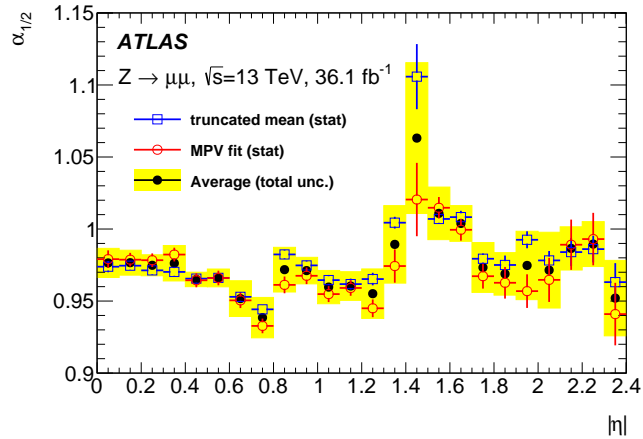
Figure 5: Ratio \alpha_{1/2} = (\langle E_1 \rangle^{\text{data}} / \langle E_1 \rangle^{\text{MC}}) / (\langle E_2 \rangle^{\text{data}} / \langle E_2 \rangle^{\text{MC}}) as a function of |\eta| , as obtained from the study of the muon energy deposits in the first two layers of the calorimeters. The results from the two methods are shown with their statistical uncertainties. The final average measurement is shown with its total uncertainty including the statistical and systematic uncertainties.
