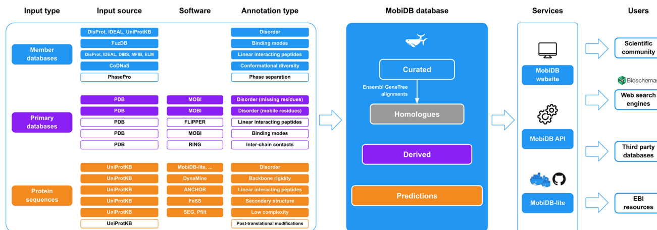
Figure 1. MobiDB data and services. The MobiDB pipeline (left) includes the input source, output features and software used to generate MobiDB data (center). Different background colors indicate different levels of annotation quality. White background in the pipeline (left) indicates novel features, databases and software integrated into MobiDB v4. MobiDB data can be accessed through a website and an API (right). MobiDB predictions can be generated using the MobiDB-lite software which is available both as a Docker container and as a Python package from GitHub. MobiDB web pages are decorated with BioSchemas profiles which allows external search engines to retrieve disorder annotations exploiting structured data.
