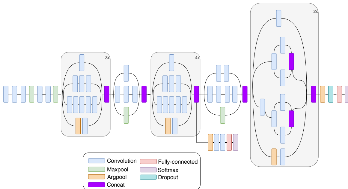
Figure 9. Inception architecture [21].
