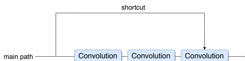
Figure 5. Residual block.
