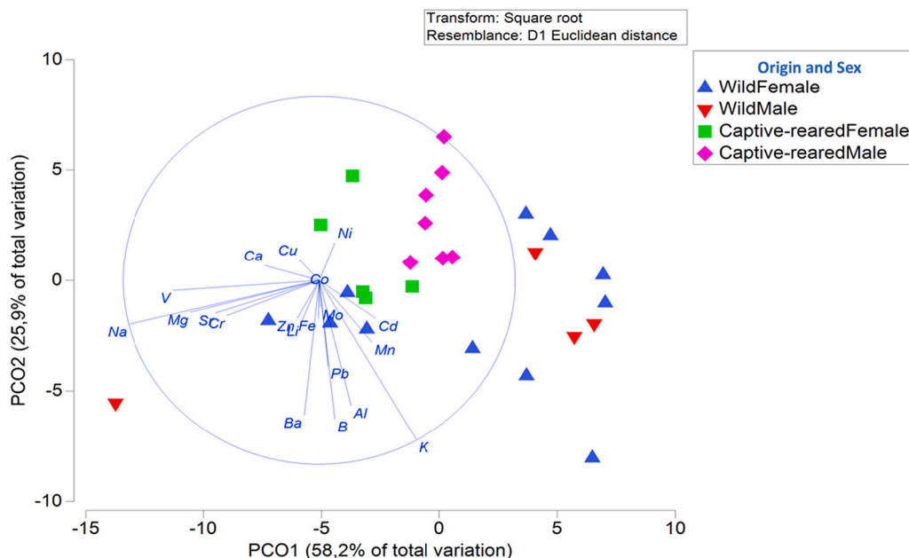
Fig. 2. Principal coordinate analysis (PCoA) showing the first two axes (84.1% of variability) based on Euclidean distances of square-root-transformed values of the heavy metals and trace elements content in the muscle of fish groups with factors (origin and sex).
