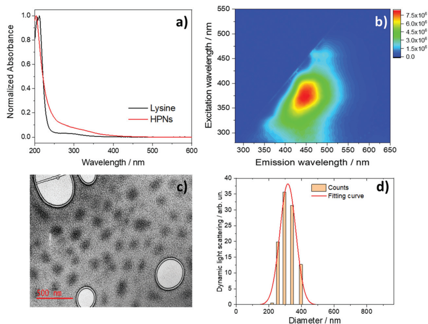
Fig. 2 (a) UV-Vis absorption spectra of lysine (black line) (0.01 M) and carbon nanomaterials (red line) in water (250 \mu\text{g mL}^{-1} ). (b) The excitation (y axis)–emission (x axis)–intensity (false colour scale) fluorescence map of the carbon nanomaterials in water (0.25 \text{mg mL}^{-1} ). (c) Representative bright-field TEM image of HPNs. (d) Dynamic light scattering of the HPNs (black spots) in water (250 \mu\text{g mL}^{-1} ). The bright areas are holes in the TEM grid.
