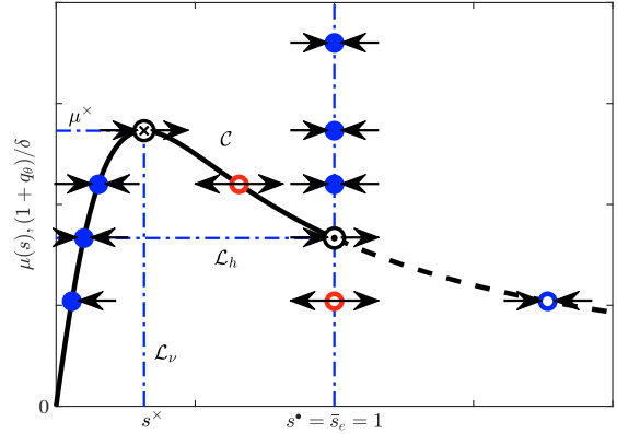
Fig. 1. Intersection of the three curves defined in (12) with their respective stability properties and bifurcation concentrations s^\times, s^\bullet .
