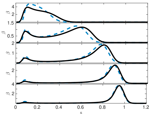
Fig. 2. Snapshots at t \in \{1, 2, 3, 4, 5\} of the marginal PDF \beta for multiplicative noise (black line) with q_\theta = 0.004 and additive noise (blue line) with intensity q = 0.002 .
