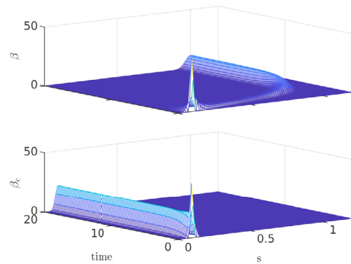
Fig. 3. OL (top panel) and CL (bottom panel) marginal state substrate evolution with \delta^* = 21.11 , initial conditions: (m_0, s_0) = (0.9, 0.0901) , background noise intensity: (q_m, q_s) = (0.002, 0.002) , inlet flowrate noise intensity q_\theta = 0.004 and control gain k = 8 .
