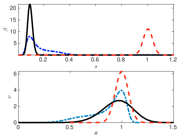
Fig. 4. Stationary marginal substrate PDF \bar{\beta} (top panel) and stationary control variable PDF \nu (bottom panel). Initial conditions: (m_0, s_0) = (0.9, 0.0901) , noise: (q_m, q_s) = (0.002, 0.002) , q_\theta = 0.004 , \delta^* = 21.11 , Set point: \bar{s} = 0.0901 , k = 2 blue line; k = 8 black line; OL dashed red line.
