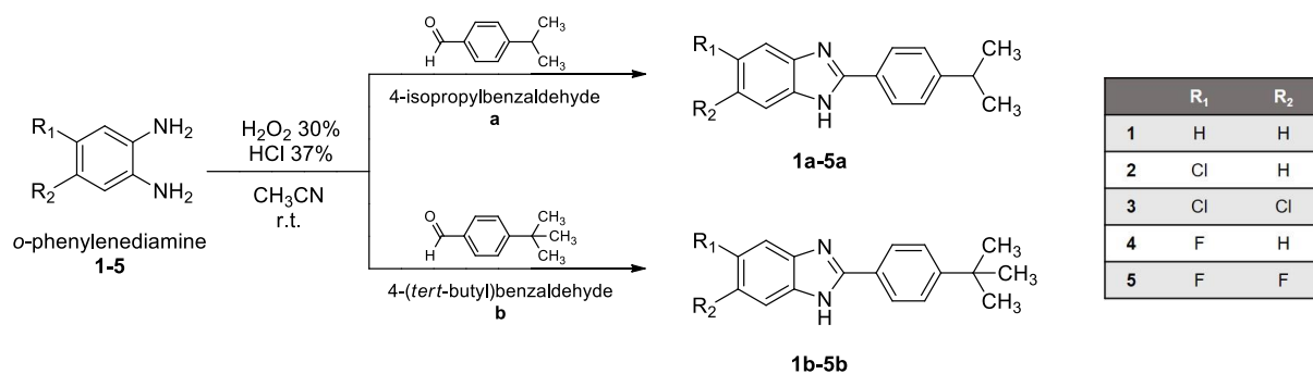
Scheme 1. 1a,b-5a,b .
