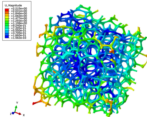
Fig. 21 Displacements of RVE in the prediction of D_{33} parameter
