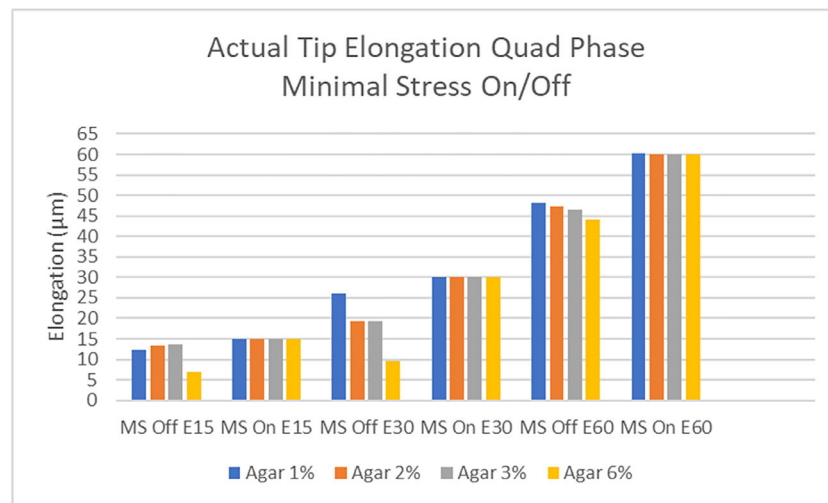
Figure 3. Actual tip elongation in quadrant removal mode with feedback control off or on when nominal elongation (requested elongation) was set to 15 \mu\text{m} (E15), 30 \mu\text{m} (E30), or 60 \mu\text{m} (E60). Colored bars indicate increasing agar gel percentage.
