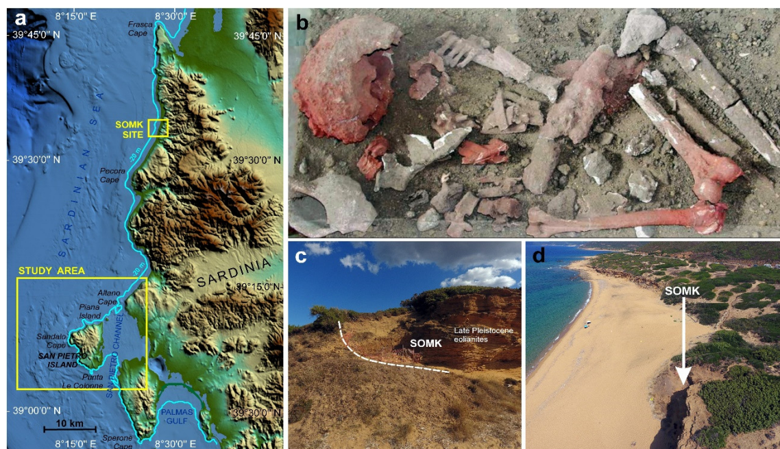
Figure 15. Mesolithic man in Sardinia west coast: (a) Location of S'Orku e S'Orku (SOMK) site and study area, palaeo-coastline of Mesolithic period (9 kyr BP) at 20 m. (b) The heavily ochre-stained skeletal remains (after Melis and Mussi, 2016 [81]). (c) View of SOMK Mesolithic site. (d) General view of the present-day position of Mesolithic SOMK site along the Sardinian west coast.
