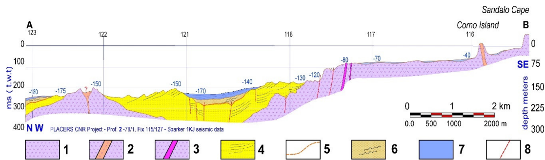
Figure 4. Geological section from seismic data of: Oceanography and Seabed - Mineral Resources - PLACERS Project CNR—Profilo 2-78/1, Fix 115/127—Sparker 1KJ: (1) Volcanites (Lower-Middle Miocene); (2) emission chimney; (3) dikes; (4) marine sedimentary sequence with inclined reflectors (Middle-Upper Miocene); (5) Messinian erosional surface; (6) marine sedimentary sequence with undulated reflectors. (Pliocene-Pleistocene); (7) Holocene-current drape; (8) fault.
