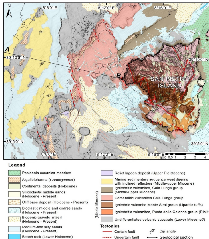
Figure 3. Geolithological sketch map of study area from the Geological Map of Italy. Scale 1:50,000—Sheet 563 “Isola di San Pietro” (Rizzo et al., 2015 [35]).
