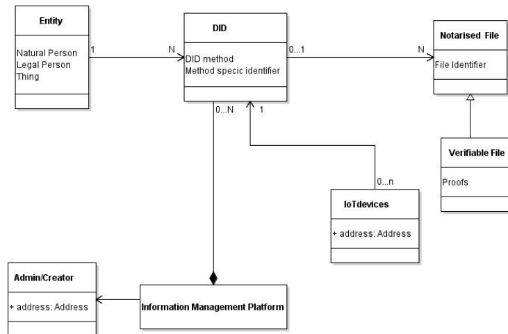
Figure 4. Class Diagram of the whole system without taking into account the methodology used for its implementation.
