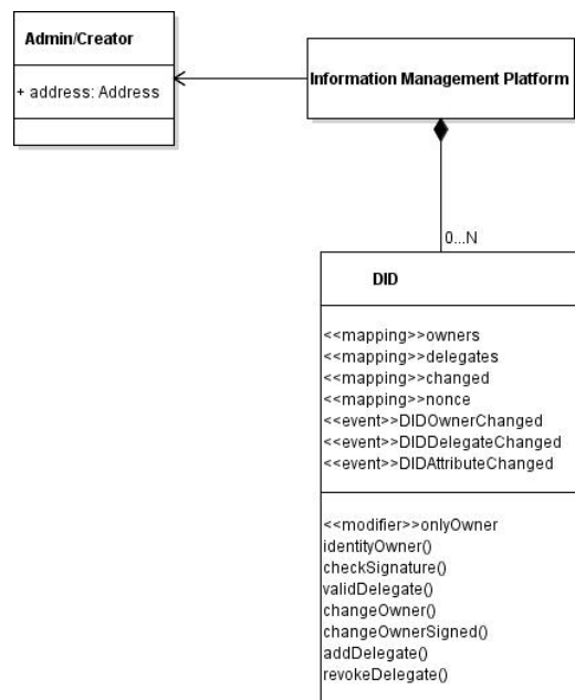
Figure 7. Class diagram of the whole system proposal.
