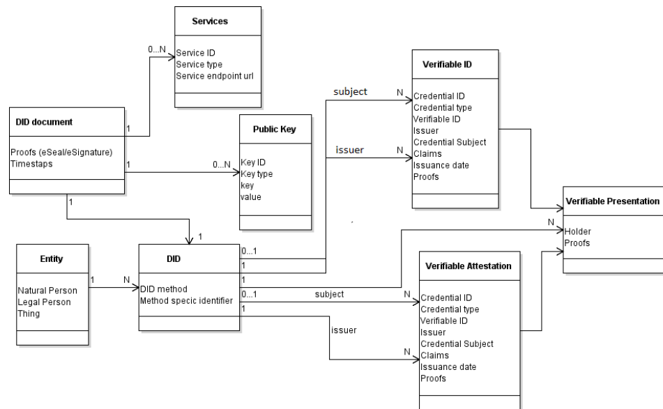
Figure 1. SSI data model proposed by EBSI.
