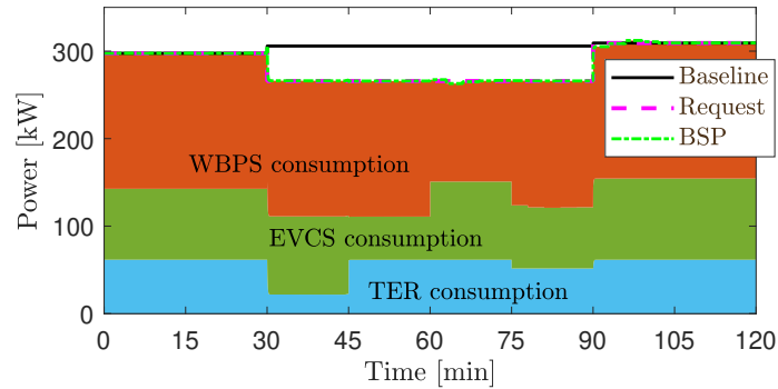
Figure 7: BSP performance in Frequency restoration operation, ( Case 1.a ).
