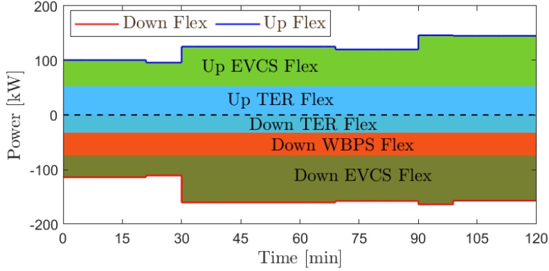
Figure 6: Flexibility of the BSP.
