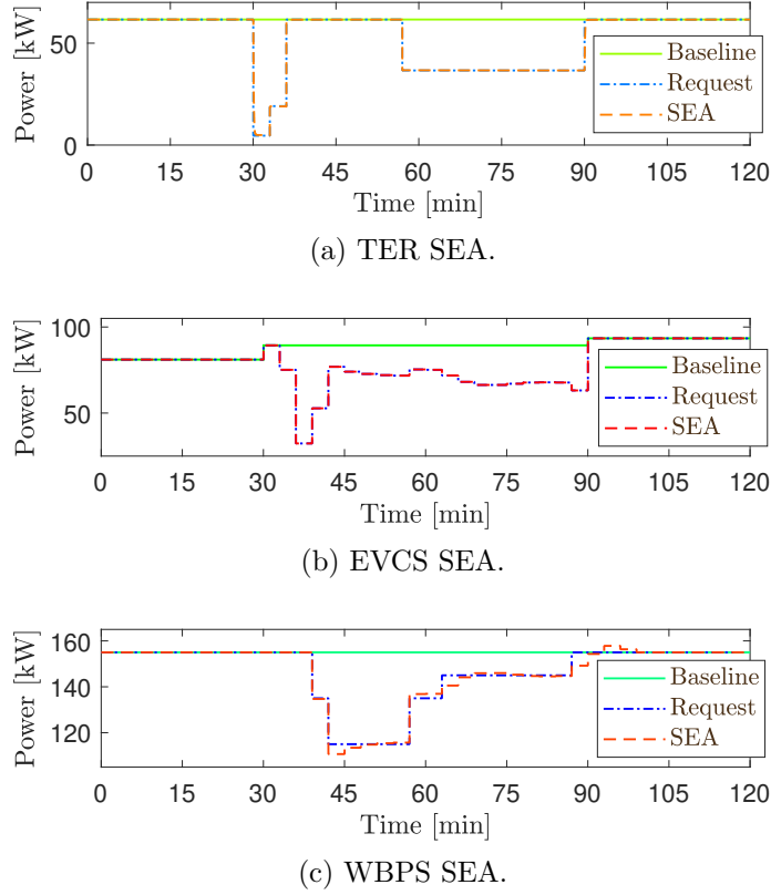
Figure 11: Single aggregator response in Frequency restoration operation for Case 1.b .
