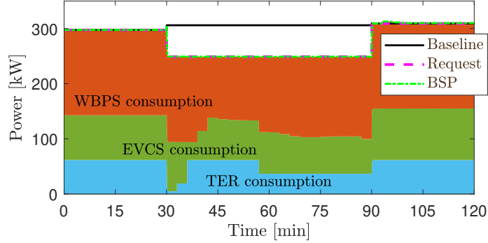
Figure 10: BSP performance in Frequency restoration operation, ( Case 1.b ).
