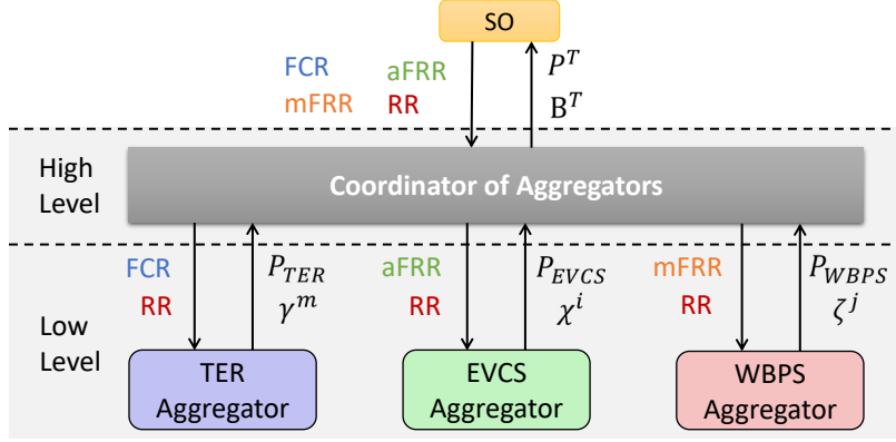
Figure 4: Two-level BSP structure: case study.
