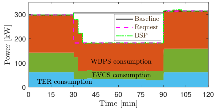
Figure 13: BSP performance in Frequency restoration operation ( Case 2 ).
