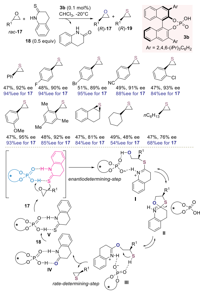
Scheme 7. TRIP-Catalyzed Kinetic Resolution of Terminal Epoxides to Thiiranes
