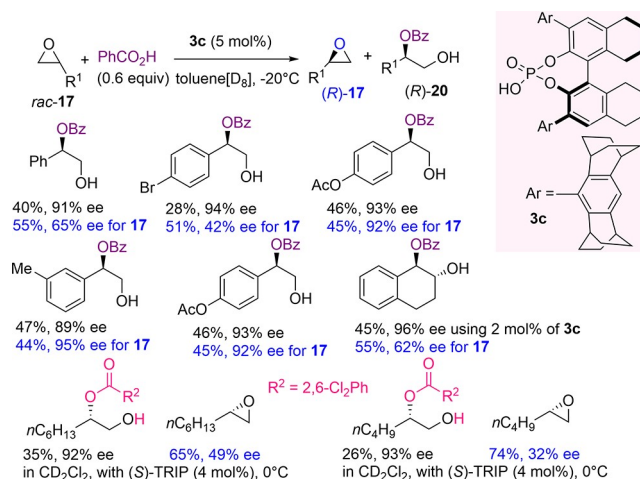
Scheme 8. \text{H}_8 -BINOL-Derived Phosphoric-Acid-Catalyzed Kinetic Resolution of Racemic Terminal Epoxides with Carboxylic Acids
