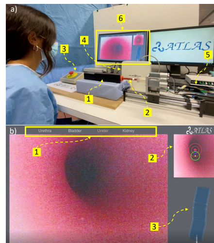
Fig. 1. a) General perspective of the Multi-level-assistance robotic platform including: 1) ureter phantom, presenting the visual conditions of a real ureter; 2) built robotic endoscope; 3) emergency stop button; 4) EM tracking system; 5) FBG interrogator and 6) Human Machine Interface. b) The Graphical User Interface: 1) current phase of the procedure; 2) processed output (center of the ureter) of our visual-servoing module and 3) 3D shape of the endoscope relative to the phantom expressed in the EM coordinate frame.
