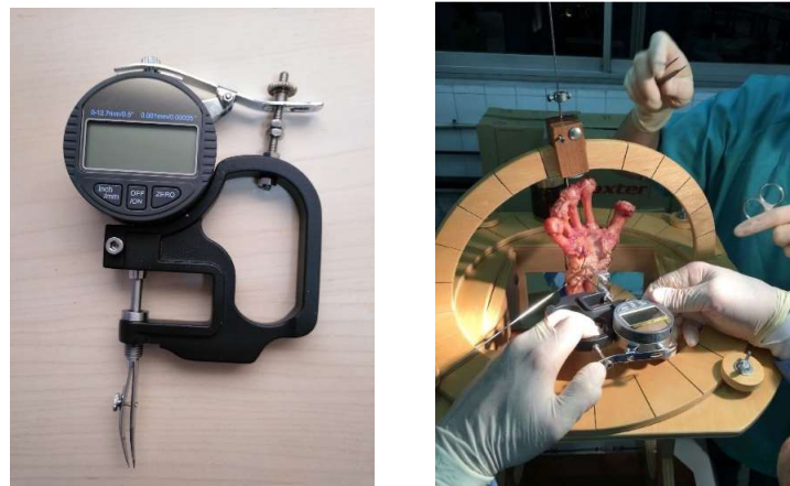
Figure 6. Left, apparel to measure the ligament displacement. Right, jig designed by physicians of Universitat Autònoma de Barcelona (UAB).
