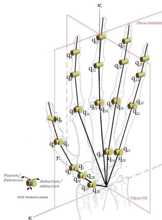
Figure 2. Dorsal view right hand model.
