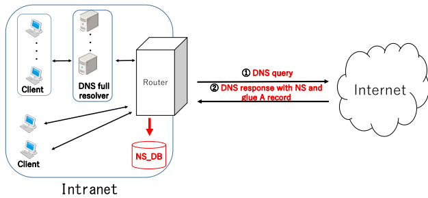
Fig. 10 DNS data collection in case of DNS response with NS and glue A record.
