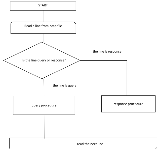
Fig. 8 The workflow of NS_DB creation program.
