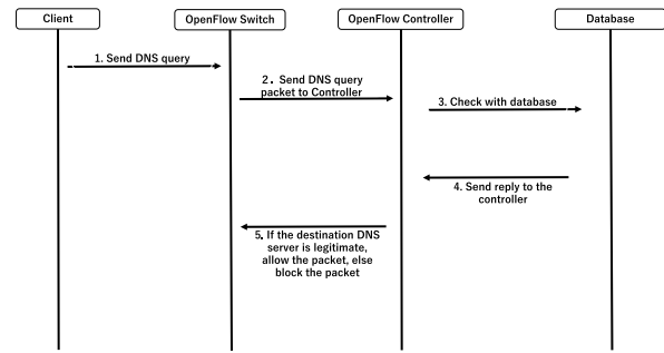
Fig. 7 Overview of the workflow in the proposed system.
