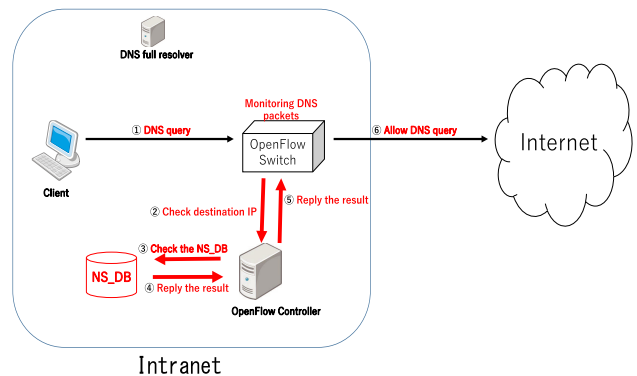
Fig. 9 The detailed procedure of the proposed system.
