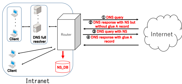
Fig. 11 DNS data collection in case of a DNS response with NS but without glue A record.
