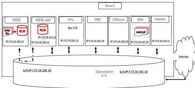
Fig. 12 The network topology used in evaluation.
