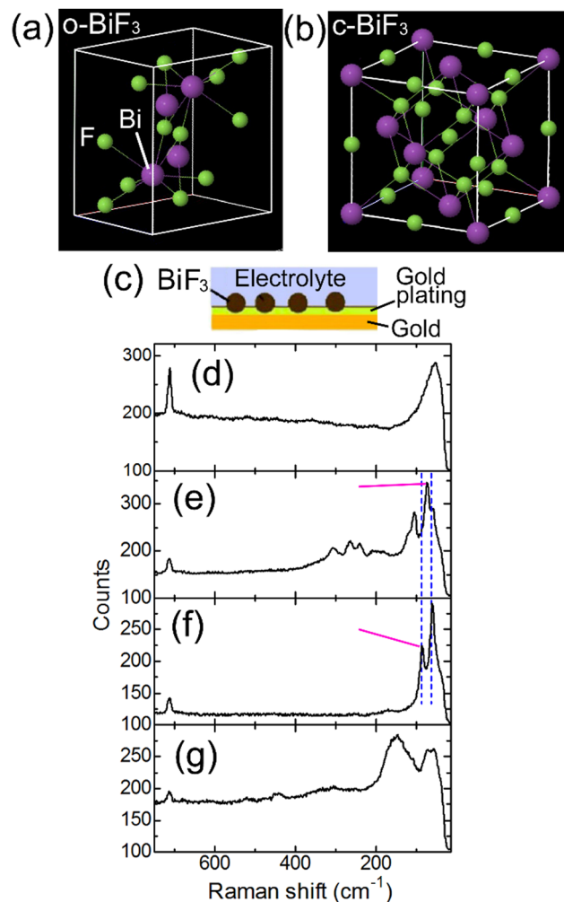
Fig. 1 Structures of o-BiF 3 and c-BiF 3 and Raman spectra of o-BiF 3 /gold and c-BiF 3 /gold samples in electrochemical cells. (a) and (b) show structures of o-BiF 3 and c-BiF 3 , respectively. (c) shows an illustration of an o-BiF 3 /gold or a c-BiF 3 /gold sample. (d) and (e) show Raman spectra obtained at the positions of the gold substrate and an o-BiF 3 particle on an o-BiF 3 /gold sample in a cell before defluorination, respectively. (f) shows a Raman spectrum obtained at the position of a particle on the o-BiF 3 /gold sample in the cell after defluorination. (g) shows a Raman spectrum obtained at the position of a particle on a c-BiF 3 /gold sample in another cell before defluorination.
