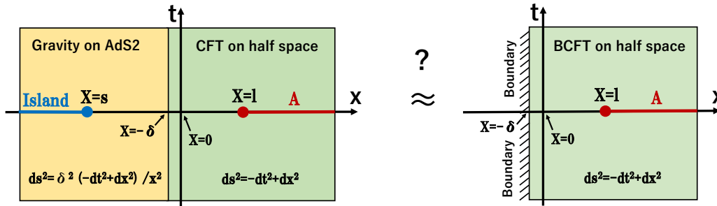
Figure 2. A sketch of setup of calculating entanglement entropy when we couple a CFT on a half line to a gravity on \text{AdS}_2 (left) and an equivalent setup in BCFT (right).
