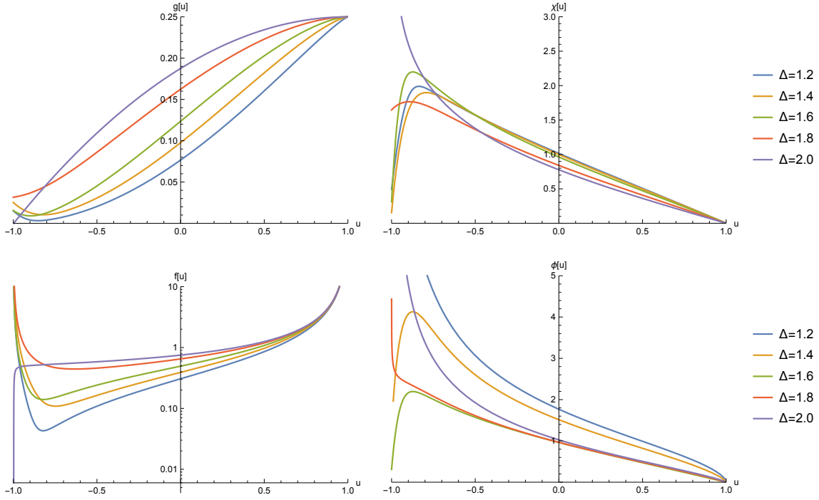
Figure 5. Numerical plots of non-singular solutions of g(u) , \chi(u) , f(u) and \phi(u) with \Delta = \Delta_+ for various dimensions in the range of 1.2 \leq \Delta_+ \leq 2.0 . At least, adjusting the values of \alpha , we can find a non-singular solution for a wide range of non-irrelevant dimension \Delta . Here we took \alpha = 2.101 (for \Delta = 1.2 ), \alpha = 2.083 (for \Delta = 1.4 ), \alpha = 1.962 (for \Delta = 1.6 ), \alpha = 1.663 (for \Delta = 1.8 ) and \alpha = 1.414 (for \Delta = 2.0 ).
