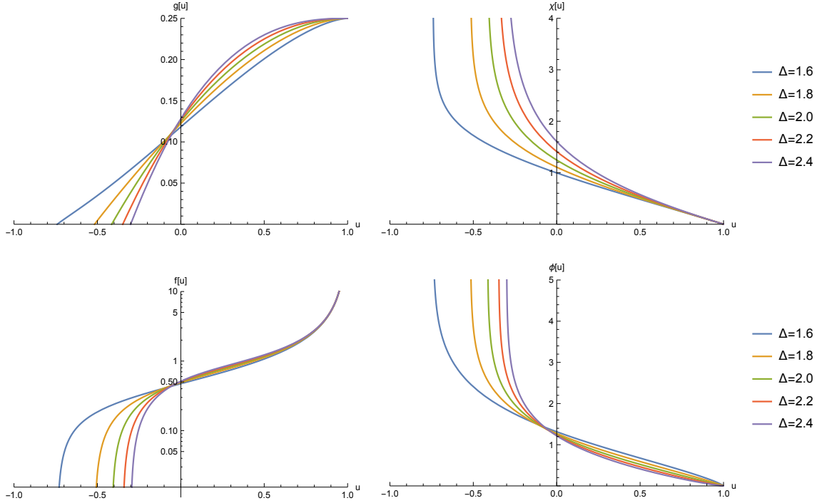
Figure 4. Numerical plots of singular solutions of g(u) , \chi(u) , f(u) and \phi(u) with \Delta = \Delta_+ for various dimensions in the range of 1.6 \leq \Delta_+ \leq 2.4 . Here we have Log plot for f(u) and choose the parameter \alpha = 2.0 .
