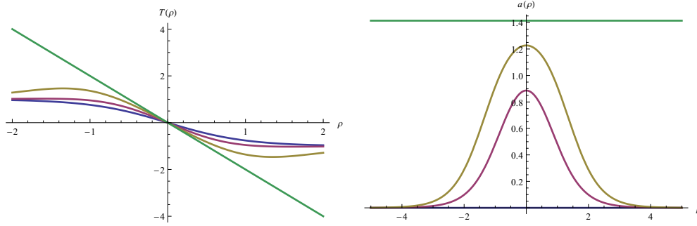
Figure 3. The tension parameter T (left) and the boundary condition parameter a (right) as functions of \rho for fixed values of \gamma . The blue, red, yellow and green curves correspond to \gamma = 0 , \gamma = 0.9/\sqrt{2} , \gamma = 0.99/\sqrt{2} and \gamma = 1/\sqrt{2} , respectively. We set \phi_0 = 0 .
