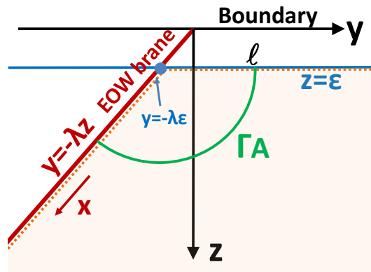
Figure 1. A sketch of AdS/BCFT setup.
