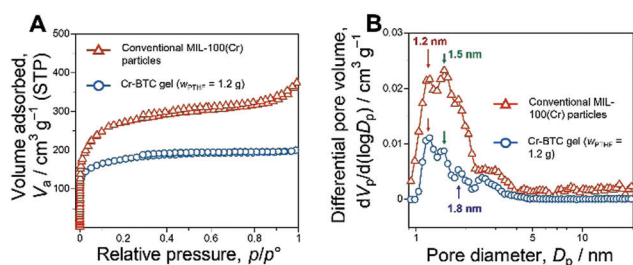
Fig. 3 Micro-/mesoporous structures of the as-dried macroporous Cr-BTC gel and the conventional MIL-100(Cr) particles. (A) Nitrogen adsorption–desorption isotherms of the samples and (B) pore size distributions obtained by NLDFT analysis. The BET surface area of conventional MIL-100(Cr) particles is calculated to be 1050 \text{ m}^2 \text{ g}^{-1} .
