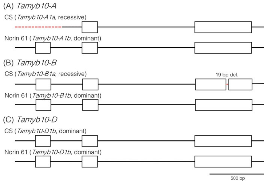
Fig. 7 Schematic features of Tamyb10 sequences of CS and Norin 61. (A) Tamyb10-A1 . CS has the recessive allele ( Tamyb10-A1a ), characterized by a large deletion, including the start codon. Norin 61 has the (wild type) dominant allele ( Tamyb10-A1b ). (B) Tamyb10-B1 . The CS has the recessive allele ( Tamyb10-B1a ) has a 19-bp deletion and Norin 61 has the dominant Tamyb10-B1b allele. (C) Tamyb10-D1 . Both CS and Norin 61 have the identical dominant allele ( Tamyb10-D1b ). The boxes indicate CDSs. The red dashed lines show the sequence polymorphisms between CS and Norin 61 assemblies.
