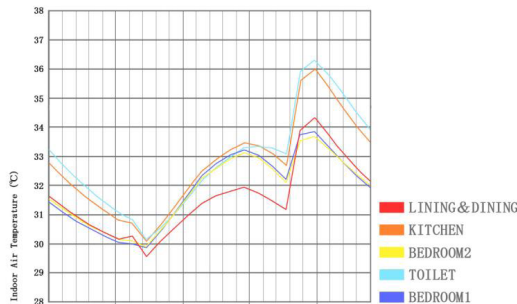
Indoor Air Temperature In The 5 spaces On May 15 OPTION 1 (WINDOWS:open from 7a. m. to 5p. m.)
