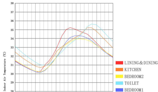
Indoor Air Temperature In The 5 spaces On May 15 OPTION 1 (WINDOWS:closed) (Trees 15m high were planted)
