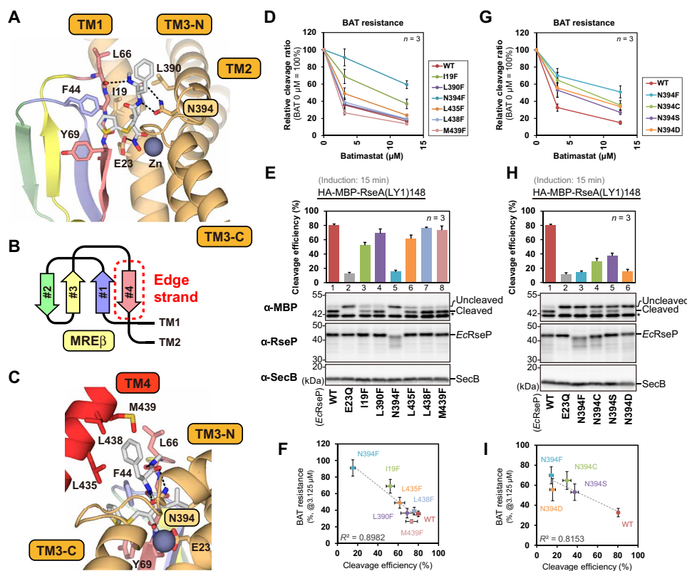
Fig. 3. Binding mode of batimastat to EcrRseP and dependence on residue N394. (A) Close-up view of the batimastat-binding site. Batimastat and the residues in direct contact with batimastat are shown as stick models. The four strands constituting the MRE \beta -sheet are shown in different colors. TM4 is omitted to visualize the binding site. (B) Topology diagram of the MRE \beta -sheet. (C) Interaction between TM4 and batimastat. (D and G) In vivo batimastat sensitivity assay. E. coli YH2902 cells harboring one plasmid for HA-MBP-RseA(LY1)148 (pYH124) and one for tagless EcrRseP (pYH825) or its variants were first treated with 0, 12.5, or 3.125 \mu M batimastat at 30°C for 10 min and then induced with 1 mM isopropyl- \beta -D-thiogalactopyranoside (IPTG) for 1 hour. The relative cleavage ratio was determined by quantitating the signal from immunoblots and comparing the value with that for the 0 mM BAT condition. Points and error bars represent the means \pm SD from three biological replicates (see fig. S7 for the raw data). (E and H) In vivo substrate cleavage assay with short induction. YH2902 cells carrying two plasmids as in (D) and (G) were incubated with 1 mM IPTG for 15 min. The cleavage efficiency was determined as described in Materials and Methods. SecB serves as a loading control. An asterisk indicates endogenous maltose-binding protein (MBP). Bar plots and error bars represent the means \pm SD from three biological replicates. (F and I) Scatterplots of the BAT resistances of the RseP mutants [relative cleavage ratio under 3.125 \mu M BAT concentration shown in (D) or (G)] against the cleavage efficiencies of the model substrate [shown in (E) or (H)].
