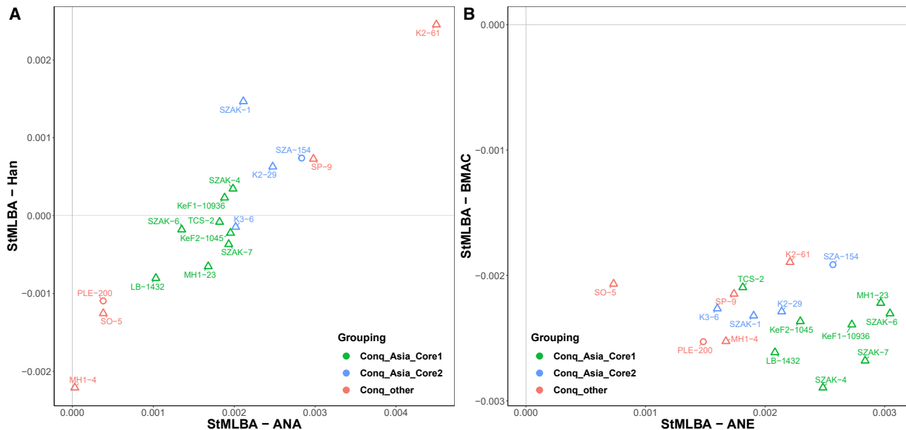
Figure 5. Two-dimensional f_4 -statistics of Conq_Asia_Core individuals
