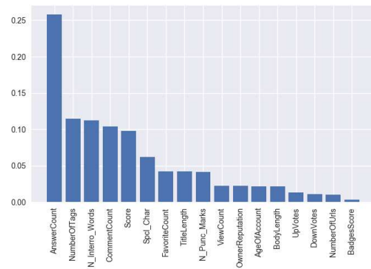
Figure 7. Feature importance graph for the topic of Ask Ubuntu .
