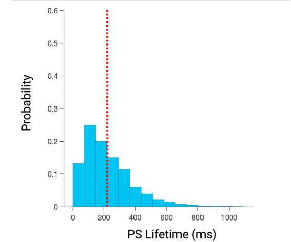
FIGURE 2 (A) The experimentally acquired data, clinically acquired data, and computational simulations utilized in this study. (B) Shows presents an example of PS detected and tracked on a phase map. (C) Demonstrates the distribution of PS lifetimes when all PS are properly sampled from an epoch of fibrillation. (D) Demonstrates the distribution of PS lifetimes when only PS present at a randomly chosen timepoint (such as the commencement of a recording) are observed.
