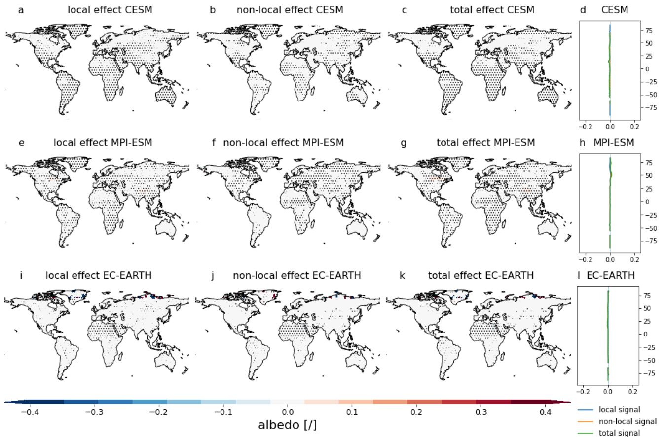
Figure E12. Annual mean albedo response to irrigation expansion (IRR-CROP) of CESM, MPI-ESM, and EC-EARTH. The local effect in CESM (a), the non-local effect (b), and the total effect (c). The latitudinal average of the local (blue), non-local (yellow), and total (green) signals of CESM (d). (e–h) Same as (a)–(d), but for MPI-ESM. (i–l) Same as (a)–(d), but for EC-EARTH. The stippling on the maps shows grid cells for which all five ensemble members agree on the sign of change.
