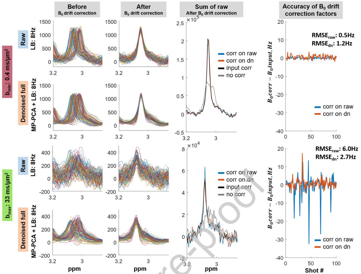
Figure 6. Spectral realignment ( B_0 drift correction) after denoising. The B_0 drift correction was performed by aligning the frequency-domain position of the tCr peak to its position on the first spectrum, using a Lorentzian apodization of 8 Hz, on raw and denoised data, for 1 MC iteration (left panels, before/after, for b_{\min} and b_{\max} ). The central panel shows the summed raw spectra with corrections derived either from the raw or the MP-PCA data, as compared to the summed raw spectra where the negative input B_0 drifts have been applied. Denoising yields no benefit of on B_0 drift correction in the case of sufficient SNR (e.g. at b_{\min} ). At low SNR (e.g. b_{\max} ), the summed raw spectra with corrections derived from MP-PCA is closely matching to the one reconstructed from the input B_0 drift values, yet with a smaller amplitude than the summed spectra with corrections from the raw data. Denoising before B_0 drift correction led to a better accuracy of the B_0 drift estimates with respect to the input drifts (right panel) at b_{\max} , and a worse accuracy at b_{\min} .
