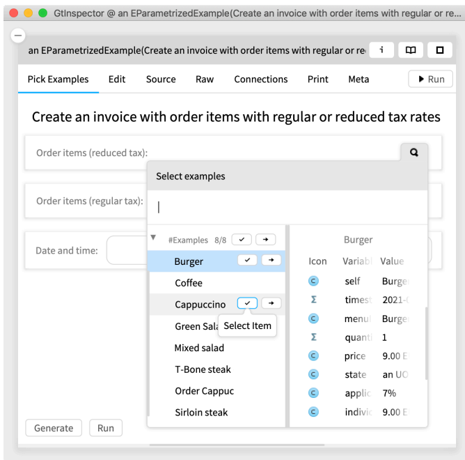
Fig. 5: A GUI to select simple domain objects
