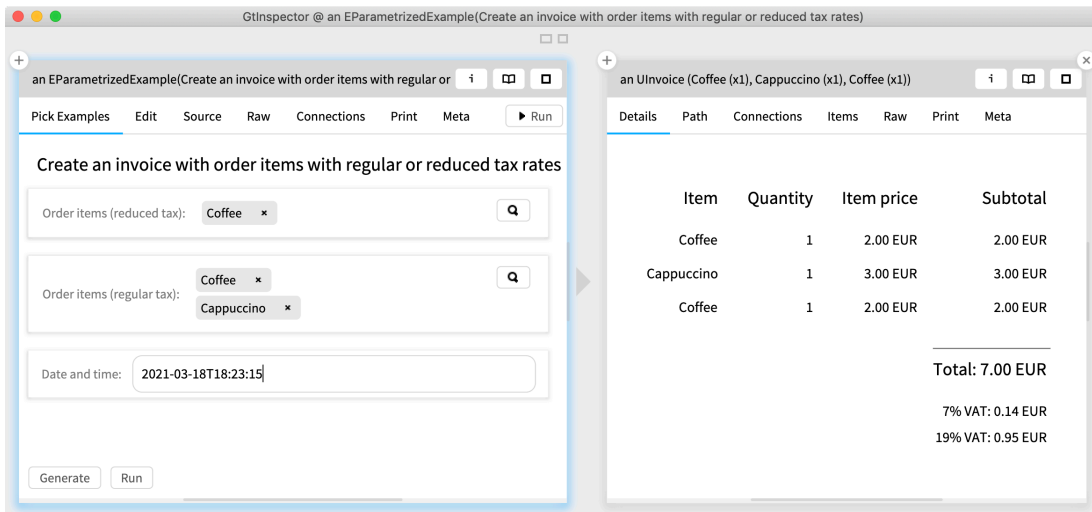
Fig. 6: A GUI to create complex domain object and explore the resulting object with printable view
