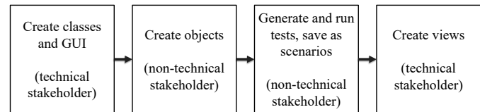
Fig. 2: Proposed BDD process
