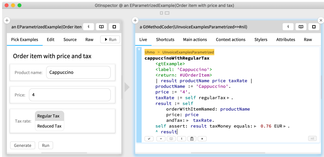
Fig. 4: A GUI to create a simple domain object and save the example as an operation
