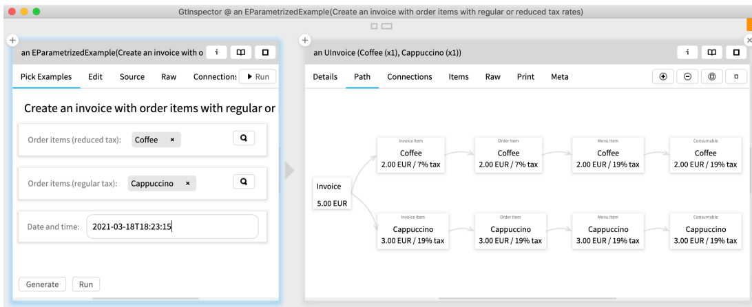
Fig. 7: A GUI to create complex domain object and explore the resulting object with composition view
