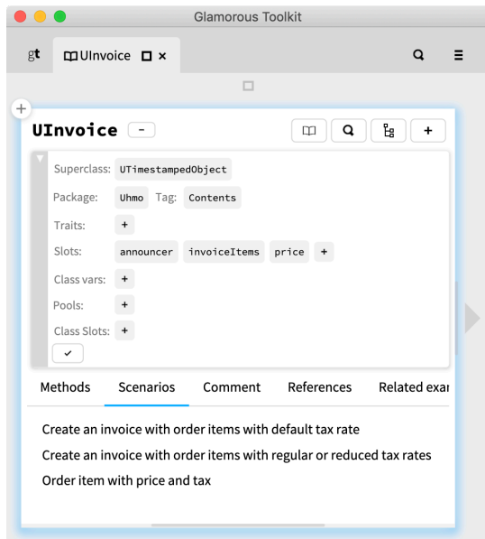
Fig. 9: Scenarios are attached to a class for efficient navigation
