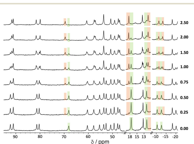
Fig. 5 1 H NMR titration experiment showing evolution of the NMR spectra of H W (0.25 mM, 298 K) in D 2 O/DMSO- d 6 (98 : 2, v/v ) on addition of increasing amounts of 1,2-DCB (number of equivalents of added guest is shown at the right-hand end of each spectrum). Some regions of the spectrum where the changes are particularly clear are highlighted in green (diminishing peaks for free H W ) and orange (emerging peaks for H W /1,2-DCB complex).
