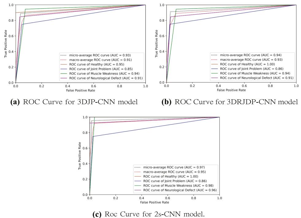
Fig. 8 Receiver operating characteristic curves for multi-class disorder classification
