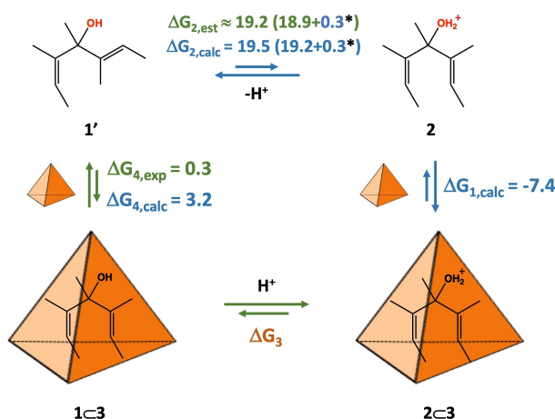
Figure 4. Thermodynamic cycle to obtain the basicity ( \Delta G_3 ) of the encapsulated reactant 1. (*) “closed” conformation of the protonated substrate is 0.3 kcal/mol higher in Gibbs energy than the most stable one. Gibbs energies in kcal/mol.
