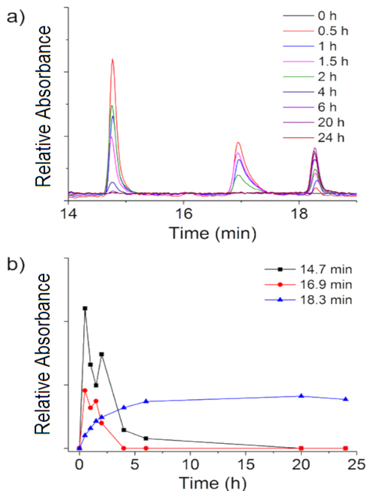
Figure 5. (a) Time-dependent HPLC chromatogram evolution under irradiation of a RuBIS CPNs colloidal suspension (200 \mu\text{g/mL} ). (b) Plot of the time-dependent variation of relative UV absorption of each component (at given retention times) upon irradiation. Detection wavelength: \lambda = 305 \text{ nm} .
